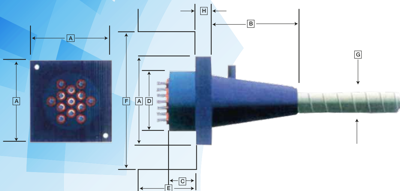
LIVE END ANCHORAGE 12.7
